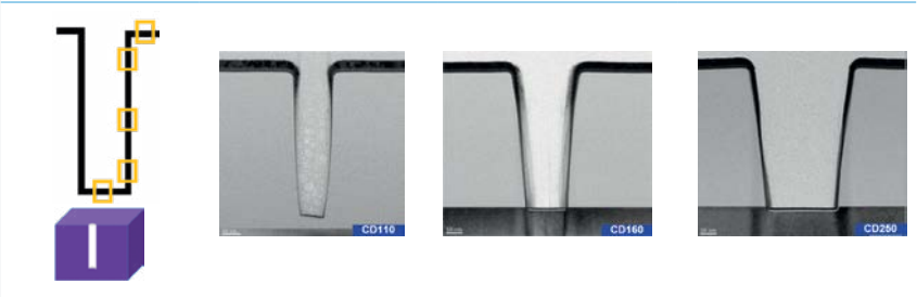
Figure 4: SDS Step coverage performance.
