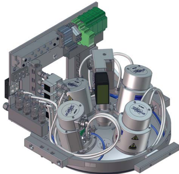
Figure 18: Drawing of the MSQ Multi-Source-Quattro with 3x sources DC/DC+ and 1x source RF/DC for co-sputtering and reactive sputtering of superconductive alloys.
