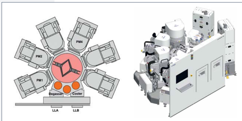
Figure 5: CLUSTERLINE® 200 system configuration for the deposition of Nb and \alpha -Ta superconductors.
