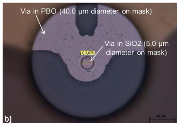
Figure 3: Fabrication process “Generation 2”: a) schematic via cross-section before PVD seed layer, and b) top view of a 5.0 μm-diameter via through SiO 2 surrounded by a 40.0 μm-diameter via through PBO.
