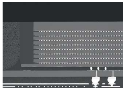
SK Hynix HBM3 – HBM DRAM die: package cross section, SEM view © Yole Group 2025
