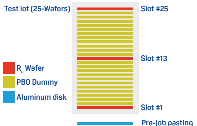
Figure 6: Procedure for the characterization of R_c stability within a 25-wafers lot. In this study, the ICP sputter etch chambers of HEXAGON are conditioned by Aluminum pasting prior processing the test lot.
