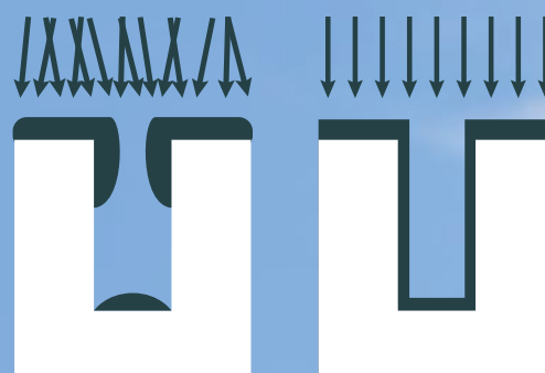
Figure 1: Conventional vs directional sputtering.
