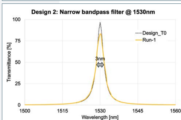
Figure 5: Transmission spectrum of a coating run of the narrow bandpass filter measured ex-situ in a spectrophotometer.
