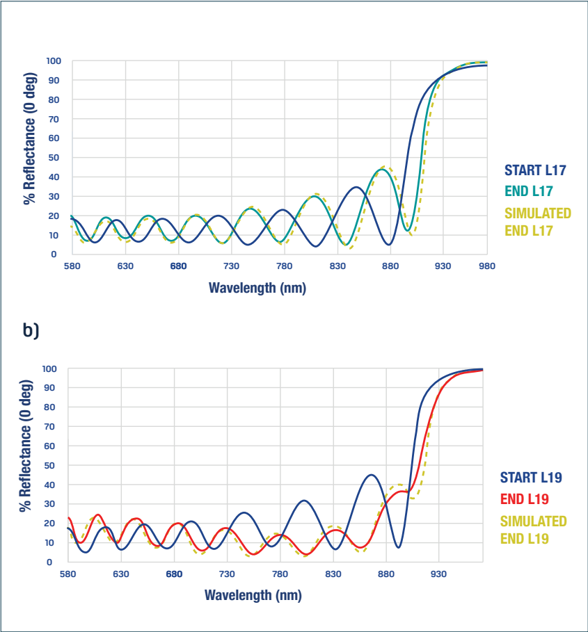
Figure 9: a) Optical monitoring spectra at start and end of the Ta 2 O 5 layer 17; b) Start and end spectra of the QNL layer 19.
