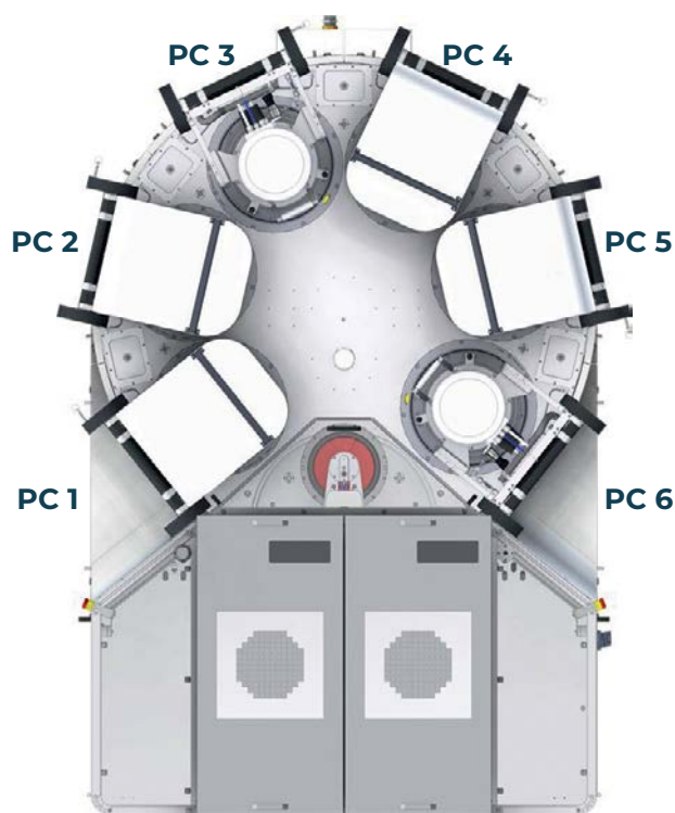
PC 1, 2, 4 & 5 ARQ 151 Target: Al PC 3 & 6 Cooling Station CS21 Cooler: Julabo FP51
