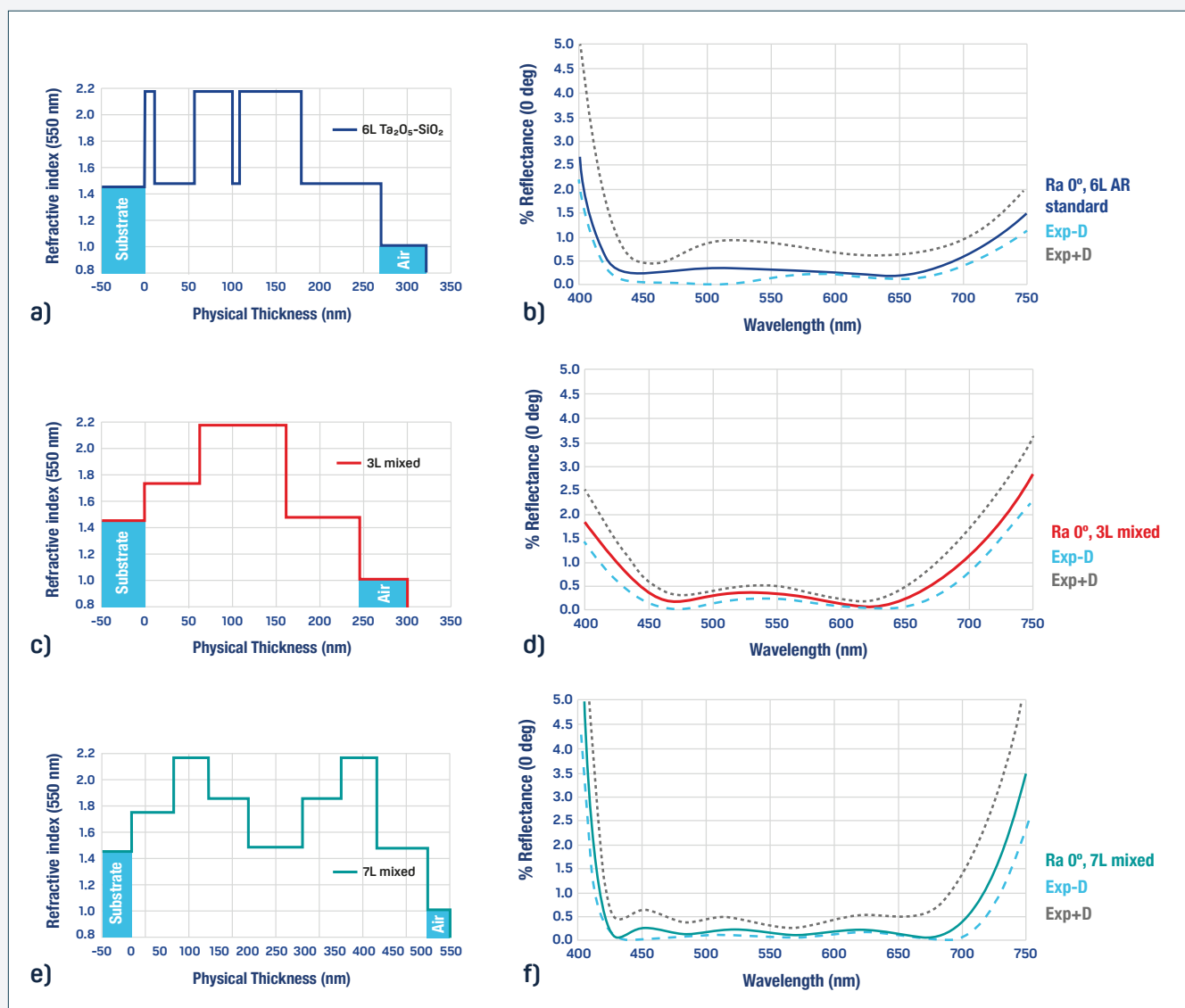
Figure 5: a,c,e) Refractive index profile of 6 layer \text{SiO}_2 to \text{Ta}_2\text{O}_5 and 3 and 7 layer designs using QNL, b,d,f) expected deviation ( 1\sigma ) of the respective designs due to thickness and refractive index deviations.
