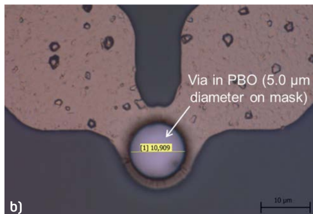
Figure 2: Fabrication process “Generation 1”: a) schematic via cross-section before PVD seed layer, and b) top view of a via through PBO with 5.0 μm nominal diameter on mask. The measured opening is 10.9 μm.
