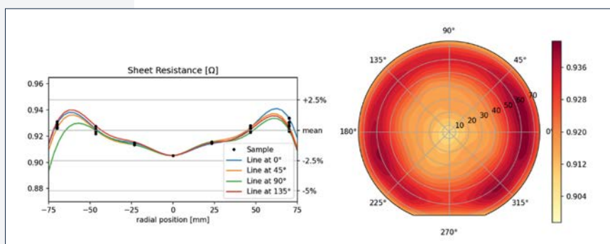
Figure 7: R_s map and uniformity of Nb 200nm deposited on 150mm silicon substrate.
