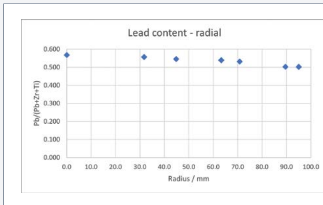
Figure 10 and 11: Radial distribution of Pb and Zr contents in at.-%.
