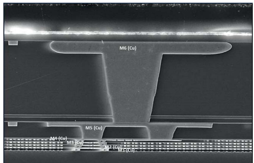
BCD 90nm Cross-Section: Thick Metal Layer In Cross-Section - Sem View Source: BCD Comparison 2024 Report, Yole Group
