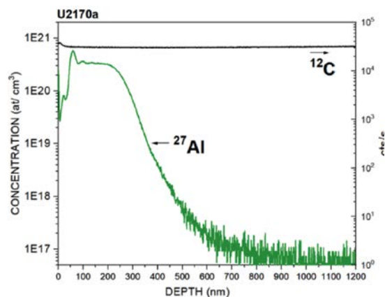
Figure 6: SIMS depth profiles were obtained on the sample implanted with Al species at 500°C. A 50 nm a-carbon layer was deposited after implantation.
