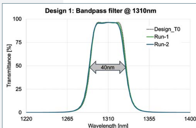
Figure 4: Transmission spectra of two coating runs of the bandpass filter measured ex-situ in a spectrophotometer. Thanks to the direct monitoring with the NIR extension, an excellent agreement with the theoretical design is achieved.
