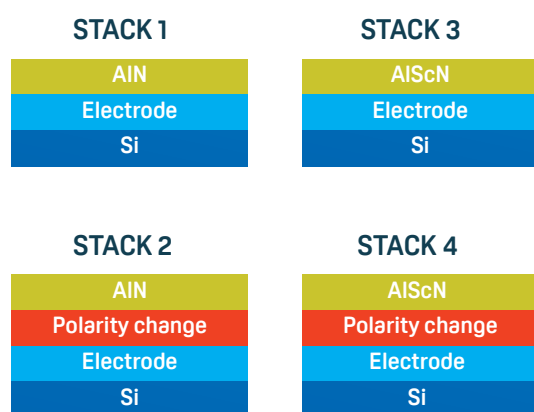
Figure 1: Stack designs for AlN and AlScN layers.
