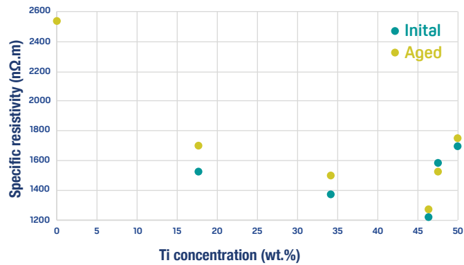
Figure 17: Aging study showing stable specific resistivity of NbTi films after “two years operation” accelerated tests, which correlates with high T_c values (see Figure 16a).
