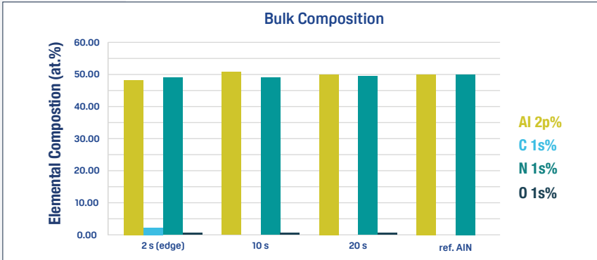
Figure 5: Elemental composition of AlN measured by XPS for different plasma times on different radial positions of the wafer. After 10s there is no C detected anymore, which is an excellent proof of high quality PEALD environment. There is only a minimal amount of oxygen detected, which is due to surface oxidation. As a reference the AlN elemental ratios (1:1) are shown.
