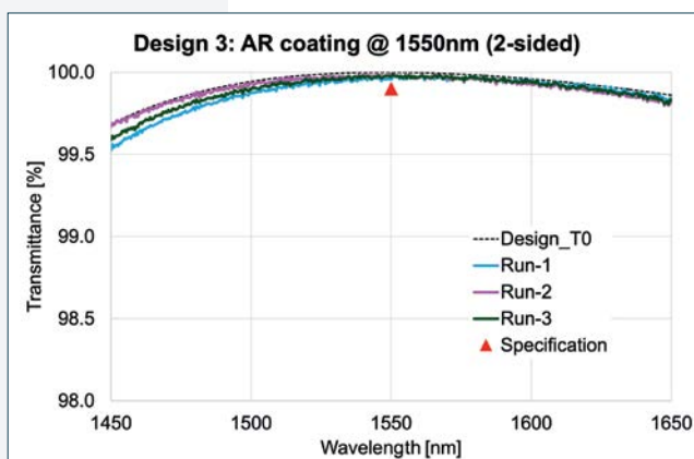
Figure 6: Transmission spectra of three substrates with an anti-reflective coating applied on both sides. Transmission >99.95% at 1550nm was achieved reproducibly.
