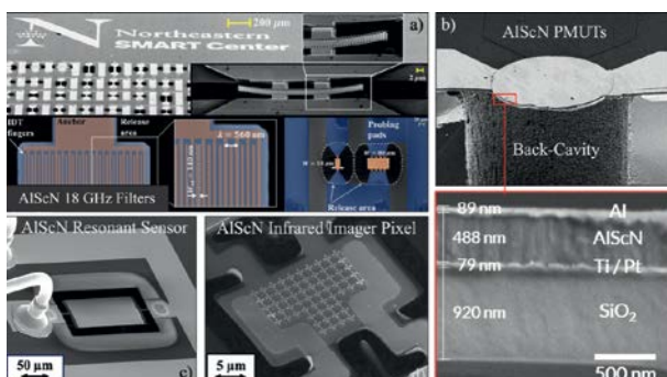
Figure 1: a) CLMR resonators for high frequency acoustic filters, b) PMUTs for intrabody ultrasonics, c) N2O resonant gas sensor, d) Infrared sensing nanoplate for imaging.
