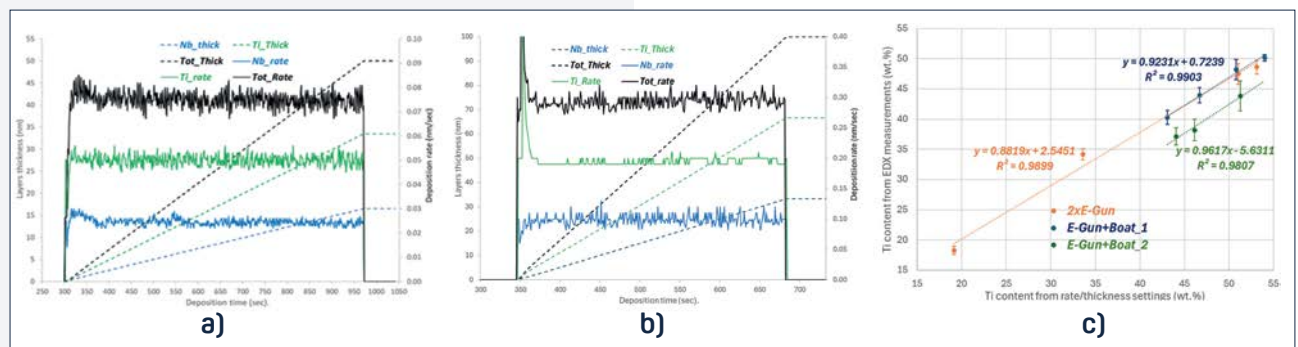
Figure 14: Adjusting of rate and thickness of co-evaporated layers with monitoring quartz crystals in double E-Guns (a) and E-Gun+Thermal Boat (b) configurations, which allows to create the corresponding process calibration curves (c).
