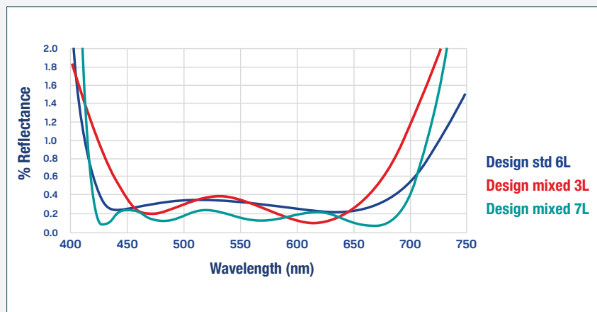
Figure 4: Antireflection designs for a standard 6 layer \text{SiO}_2 - \text{Ta}_2\text{O}_5 and 3 and 7 layer designs using QNL.
