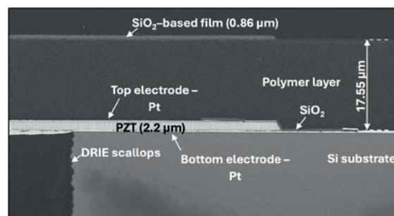
MEMS Membrane Cross-Section – SEM View
