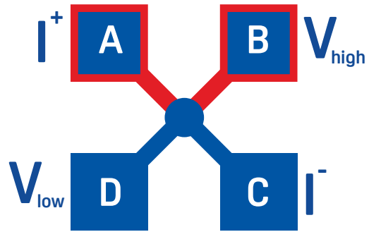
Figure 5: Electrical characterization of 4-terminals Kelvin resistors.
