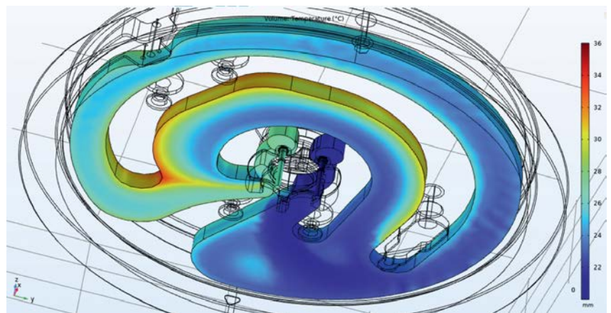
Figure 7: An advanced cooling concept was necessary to deliver a reliable solution.
