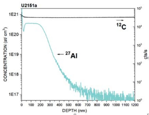
Figure 5: SIMS depth profiles were obtained on the sample implanted with Al species at 500°C. A 50 nm a-carbon layer was deposited before implantation.
