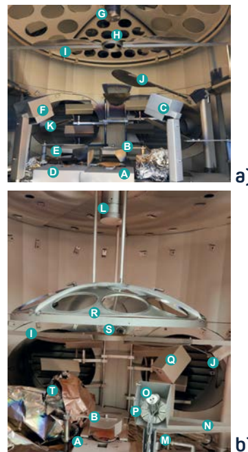
Figure 13: BAK system for depositing NbTi superconductor: double E-Guns configuration with 1050 mm sample to source distance (a); material arrangement for the co-evaporation tests (b) and E-Gun+Thermal boat configuration with 700 mm sample to source distance (c).
