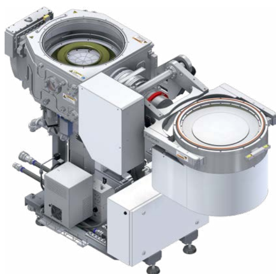
Figure 2: New RF process module for 400 mm targets integrating Very Hot Chuck and substrate bias tuning technology.
