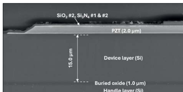
MEMS Membrane Cross-Section – SEM View
