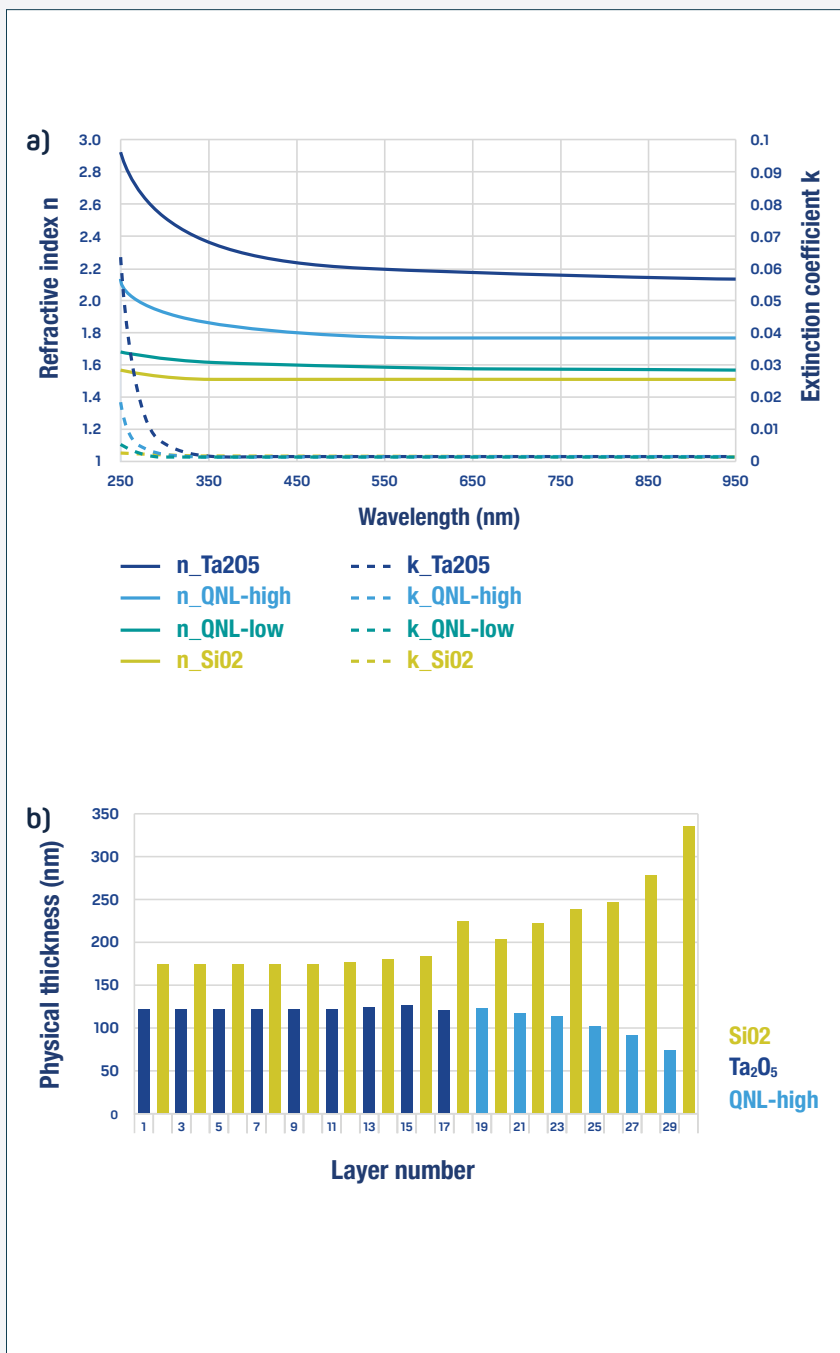
Figure 8: a) Refractive index dispersions SiO_2 , Ta_2O_5 , and of two Ta_2O_5/SiO_2 QNLs; b) Design thicknesses of a mirror for 1030nm consisting of Ta_2O_5 , SiO_2 and a QNL material.
