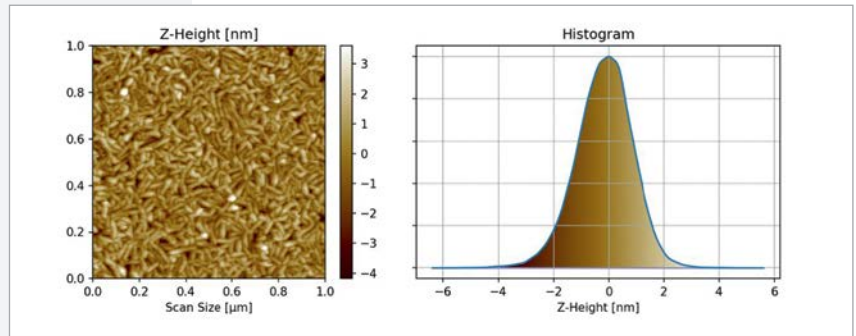
Figure 12: a-Ta 200nm film surface roughness measured by AFM in 1x1 \mu\text{m}^2 area.
