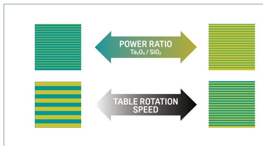
Figure 2: a) Changing the ratio of the power applied to the sputter sources allows tuning of the material composition and therefore the overall refractive index of the QNL. b) By changing the rotation speed of the substrate table, the thickness of a layer pair of the QNL deposited during each rotation can be adjusted without changing the overall material composition.
