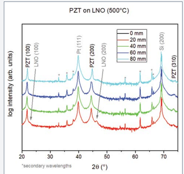
Figure 9: XRD diffractogram indicating highly textured PZT growth out-of-plane in (100)-orientation.
