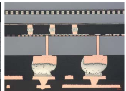
SK Hynix HBM3 – Bumps: package cross section, SEM view © Yole Group 2025
