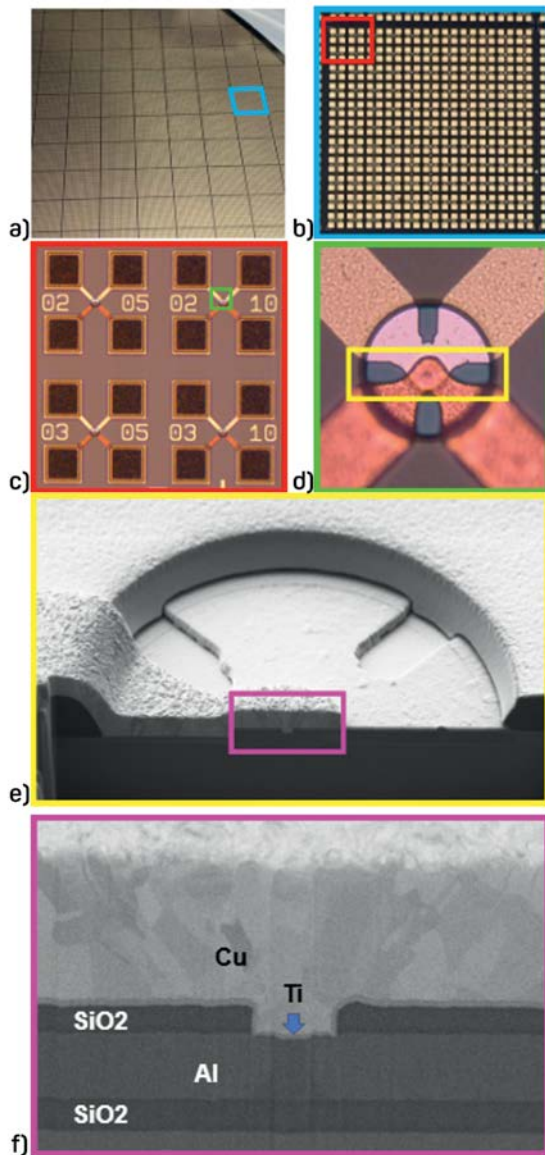
Figure 4: a) Fabricated 300 mm test wafer of “Generation 2”; b) base cell containing an array of 11 \times 11 Kelvin structures; c) example of Kelvin resistors layout; d) magnification of the contact area; e) FIB cross-section of the contact area of a 2.0 \mu\text{m} -diameter via in \text{SiO}_2 ; and f) close-up of the interface between the underlying Al and the upper Ti/Cu metallization.
