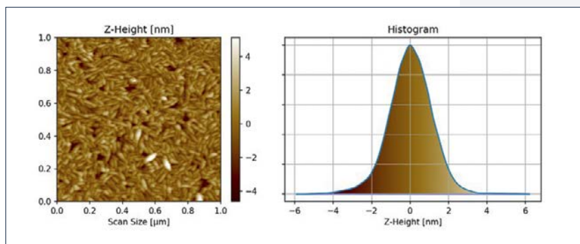
Figure 9: Nb 200nm film surface roughness measured by AFM in 1x1 mm² area.
